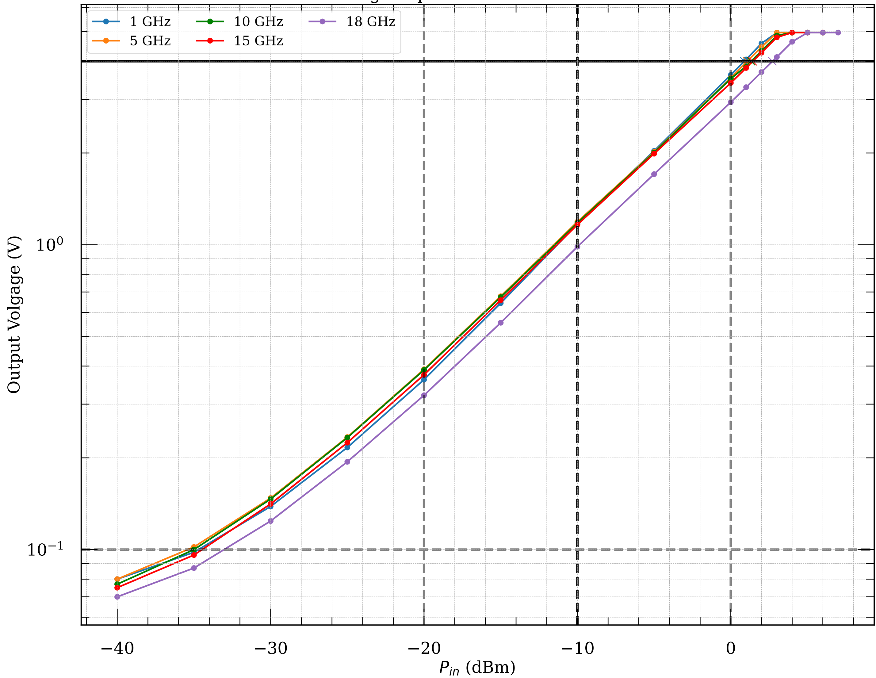
Measured voltage-to-power curve of detector module030
